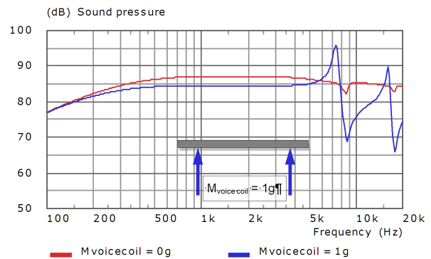
Free disk driven by 'real' force
