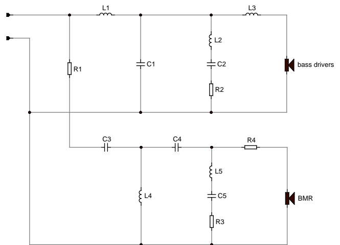
Circuit schematic of the Ovator S-400 crossover. Acoustic slopes are 4th-order Linkwitz-Riley to ensure that the drivers remain in phase throughout the crossover region
