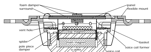
Cross-section of the Naim S-400 BMR driver
