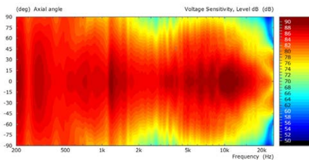
Directivity plot of a typical two-way system
