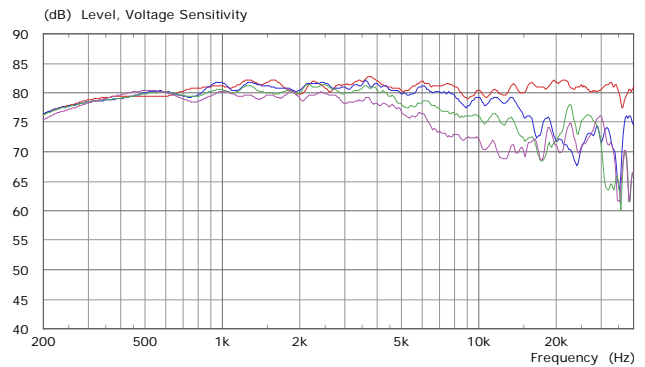
On- and off-axis response of the S-400 system
