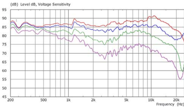
On- and off-axis response of a typical two-way system
