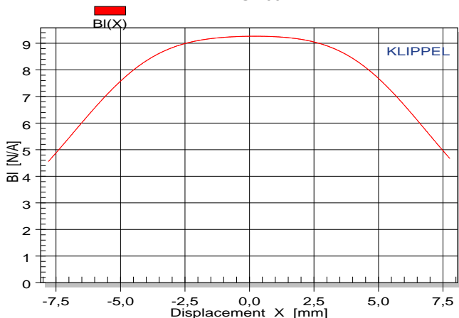
Klippel Analyzer measurement of the linearity of the S-400 bass unit's motor
