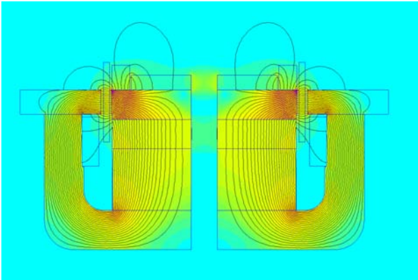
FEA model of the S-400 bass driver magnetic circuit showing the even flux density achieved in the magnet gap
