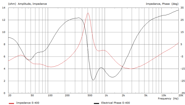
Impedance modulus (red trace) and phase (black trace) versus frequency
