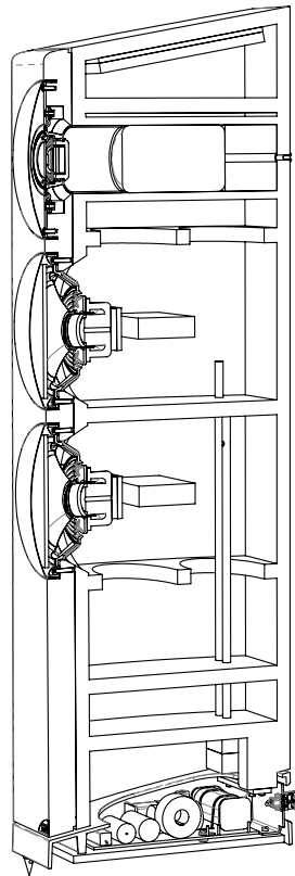
Cutaway drawing of the Ovator S-400 cabinet. Features of note include the isolated BMR module, separate enclosures for the two bass drivers and the provision of controlled 'leaks' between the latter and the external air
