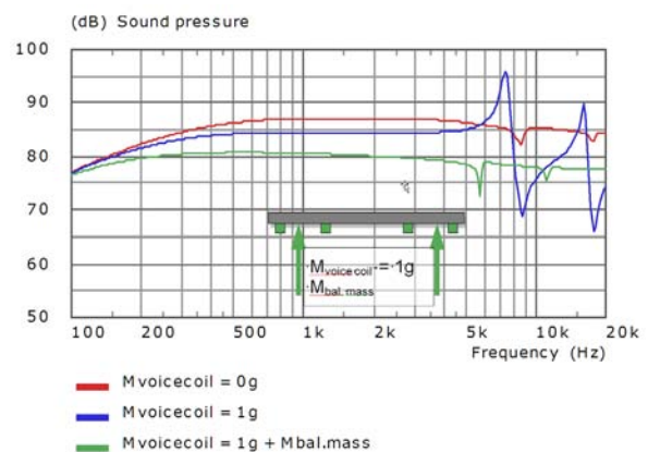
Balanced disk driven by 'real' force
