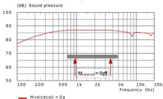
Free disk driven by 'ideal' force
