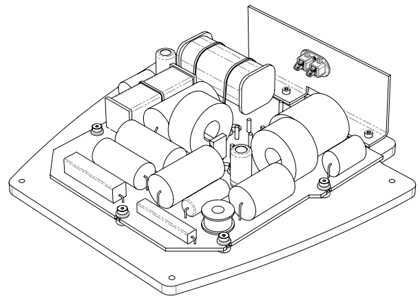
Suspended from the plinth to isolate it from vibration, the crossover module combines careful layout with meticulous choice of components
