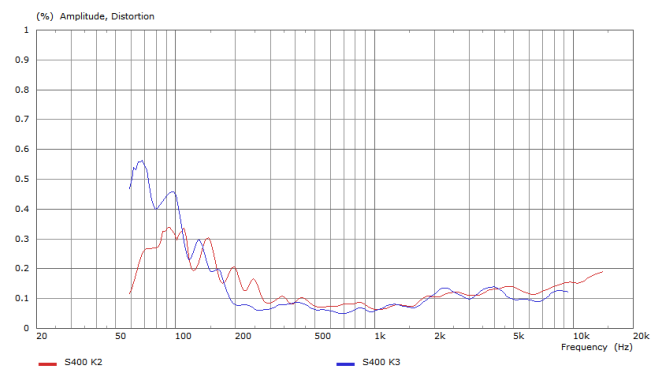
S-400 second harmonic distortion (red trace) and third harmonic distortion (blue trace)
