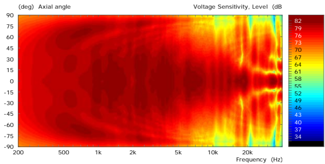
Directivity plot of the S-400 system
