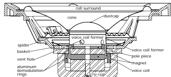
Cross-section of the S-400 bass unit
