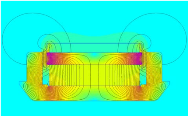
FEA model of the S-400 BMR driver magnetic circuit showing the even flux density achieved in the magnet gap
