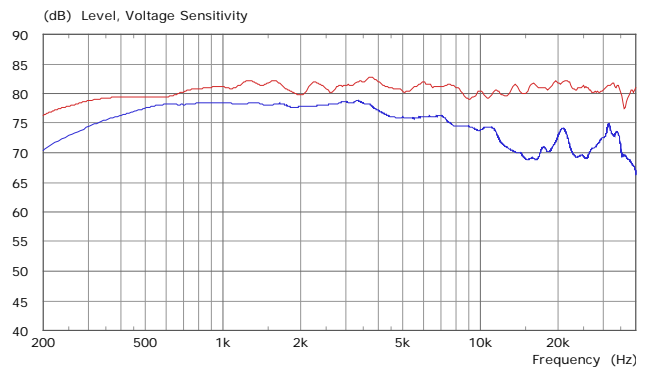
S-400 power response (blue trace) and on-axis pressure response (red trace)
